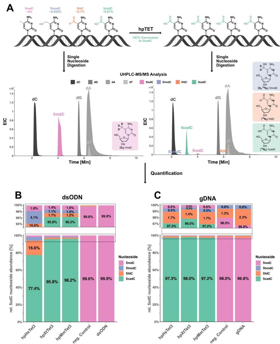
Fig. 3 Oxidation of 5mC by hpTet3-enzymes in synthetic and genomic DNA. (A) Principle of the LC-MS/MS-based quantification of 5mC, 5hmdC, 5fdC, and 5cadC in hpTet3-treated dsODN/gDNA samples and structures of used isotopologs. (B) Plot of the relative percentage of the quantified modified cytidines in the double-stranded 35-mer and (C) HEK293T gDNA following enzymatic treatment. gDNA: isolated gDNA was digested, and dC and modified dC nucleosides were quantified. As a negative control, ODN or gDNA were incubated under Tet-oxidation conditions, but without the addition of hpTet-enzymes, followed by digestion and quantification.
