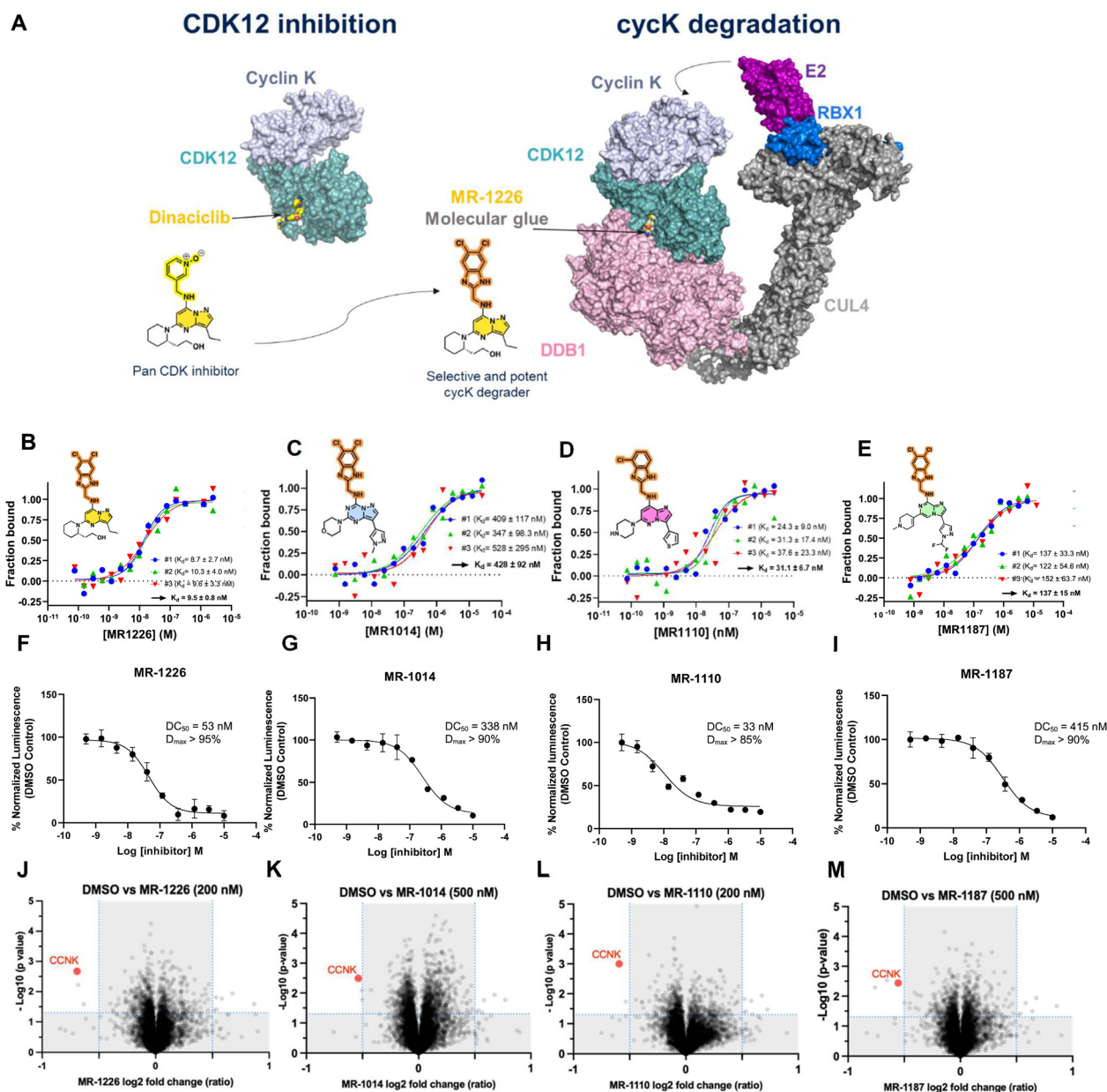
Fig. 5 Cyclin K degraders by design. (A) De novo design of cyclin K molecular glue degraders from CDK12/pan-CDK inhibitors (dinaciclilib). (B)–(E) Microscale thermophoresis studies assessing CDK12/cyclin K + DDB1 ternary complex formation induced by compound of interest. (F)–(I) Degradation of HiBiT tagged cyclin K using with MR-1187, MR-1110, MR-1014 and MR-1226 (A549 cell lines). (J)–(M) Label-free TMT-based quantitative proteomics upon treatment with MR-1187 (500 nM), MR-1110 (200 nM), MR-1014 (500 nM), MR-1226 (200 nM) at 2 h. Plot shows the significantly differentially abundant proteins ranked according to their p value (Y-axis) as -\log_{10} and their relative abundance \log_2 ratio (X axis) between DMSO control and the compound of interest. All samples were generated in triplicates and 0.5 fold changes cut off were used for avg \log_2 ratio's to analyze the data. The p values < 0.05 were considered as significant.
