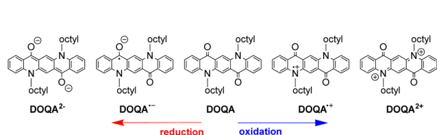
Scheme 2 Representation of oxidised and reduced forms of DOQA.
