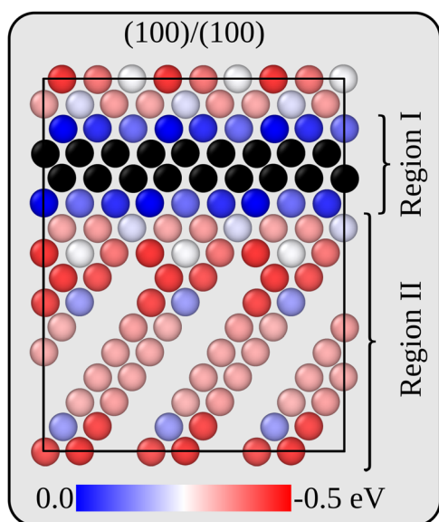
Fig. 3 Li vacancy energy profile perpendicular to interface A in the form of a color map. The plane shown in the figure contains the interface normal and the normal of the \text{VO}_2 and \text{Li}_2\text{F} planes in the \text{Li}_2\text{VO}_2\text{F} structure. Relative energies with respect to a position in the middle of the LiF phase are given from 0 (blue) to -0.5 eV (dark red).
