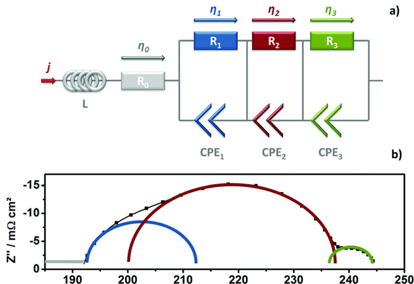
Fig. 6 (a) Diagram of the equivalent circuit used for EIS analysis; (b) illustration of a Nyquist plot displaying analyzed arcs (time constants). Reproduced with the permission from ref. 82. Copyright 2017, RSC.
