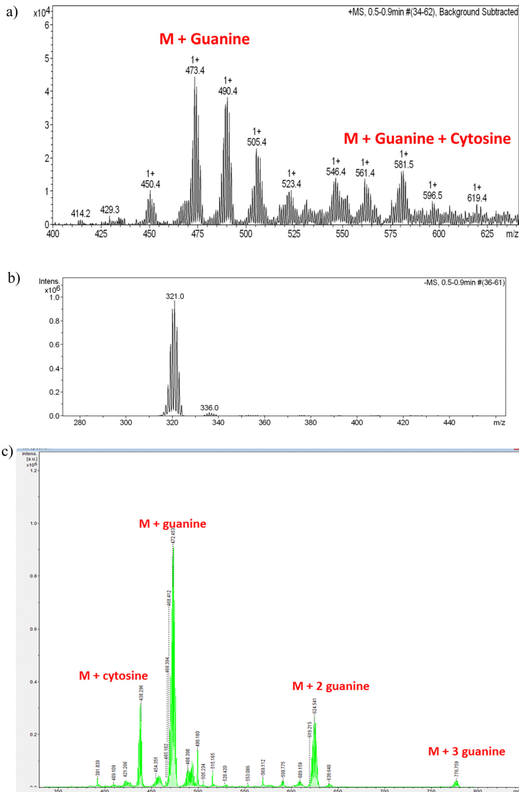
Fig. 8 (a) Magnification of the ESI-MS spectrum of the CT-dsDNA/Na[o-FESAN] nanohybrid at the positive mode in the range 400–650 m/z with isotopic (+1) distribution; Fig. S8 at the ESI ^{\dagger} displays the full spectrum in the range 0–1200 m/z . (b) ESI-MS spectrum of the CT-dsDNA/Na[o-FESAN] nanohybrid at the negative mode with isotopic (–1) distribution in the range 270–470 m/z ; only molecular peak of the [o-FESAN] ^{-} at 321.0. (c) MALDI-TOF-MS of the nanohybrid CT-dsDNA/Na[o-FESAN] using DHB (2,5-dihydroxybenzoic acid) matrix at the anode with 30% attenuation.
