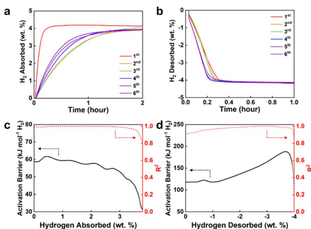
Fig. 3 Hydrogen sorption kinetics of the Mg@DL-Ti 2 CCl x composite. (a) Isothermal hydrogen absorption at 200 °C under 15 bar of H 2 and (b) hydrogen desorption at 300 °C under 0 bar of H 2 . Activation barrier for (c) absorption and (d) desorption as a function of absorbed and desorbed wt% H 2 , respectively.
