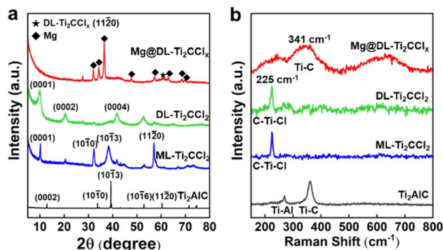
Fig. 2 Change of the crystalline and chemical structures of the Ti 2 AlC MAX phase, ML-Ti 2 CCl 2 , DL-Ti 2 CCl 2 and Mg@DL-Ti 2 CCl x composite based on (a) X-ray diffraction (XRD) patterns and (b) Raman spectra.
