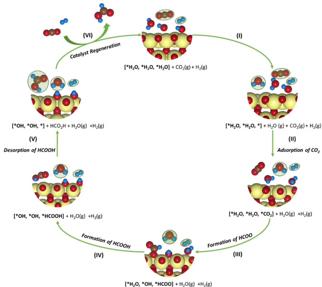
Fig. 7 Schematic representation of the plausible \text{CO}_2 reduction mechanism for the \text{SnO}_2 -based model systems. The adsorbates in gaseous states are marked in green. Color codes: Sn (yellow), C (brown), O (red), H (blue).
