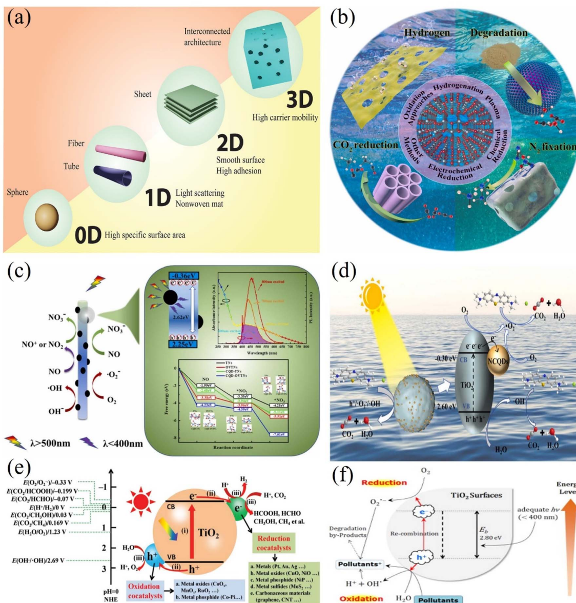
Fig. 8 (a) Various structural configurations of \text{TiO}_2 at both the nano and macro scales. Adopted from ref. 171 with permission. (b) A schematic diagram depicting the utilization of defective \text{TiO}_2 materials in photocatalytic applications. \text{TiO}_2 photocatalysts are fabricated using various methods such as hydrogenation, plasma treatment, chemical reduction, electrochemical reduction, and oxidation. Adopted from ref. 172 with permission. (c) Oxygen vacancies and carbon quantum dots (CQDs) with up-conversion properties for enhanced photocatalytic activity of \text{TiO}_2 for NO removal under visible light irradiation. Adopted from ref. 173 with permission. (d) Mechanism for the degradation of methylene blue using NCQDs/ \text{TiO}_2 under solar irradiation. Adopted from ref. 174 with permission. (e) Illustration of the photocatalytic reactions occurring on \text{TiO}_2 -based photocatalysts, enhanced with reduction and oxidation cocatalysts. The redox potentials of various species at pH = 0, referenced to the NHE, are also depicted. Adopted from ref. 175 with permission. (f) Pollutant removal through the generation of photoinduced charge carriers ( e^-/h^+ ) on the surfaces of semiconductor \text{TiO}_2 particles. Adopted from ref. 176 with permission.
