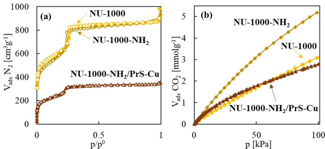
Fig. 3 Adsorption behavior: (a) N_2 adsorption–desorption isotherms at -196\text{ °C} and (b) CO_2 adsorption isotherms at 0\text{ °C} of the studied samples compared to pristine NU-1000.
