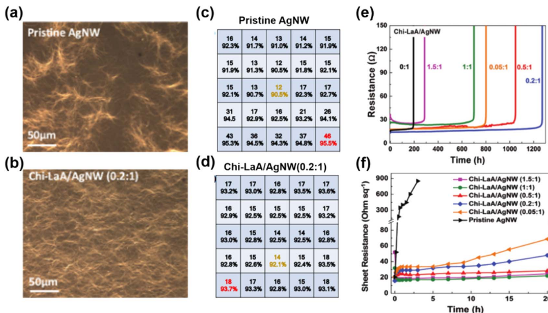
Fig. 3 The stability of the pristine Ag NW and uniform Chi-LA/Ag NW FTEs. (a and b) Optical images. (c and d) Sheet resistance and transmittance of FTEs with a size of 6 \times 6 \text{ cm}^2 . (e) Resistance as a function of time under a current of 250 \text{ mA cm}^{-2} . (f) Sheet resistance as a function of time at high temperature of 180^\circ \text{C} . Reproduced with permission. 71 Copyright 2020, the Royal Society of Chemistry.
