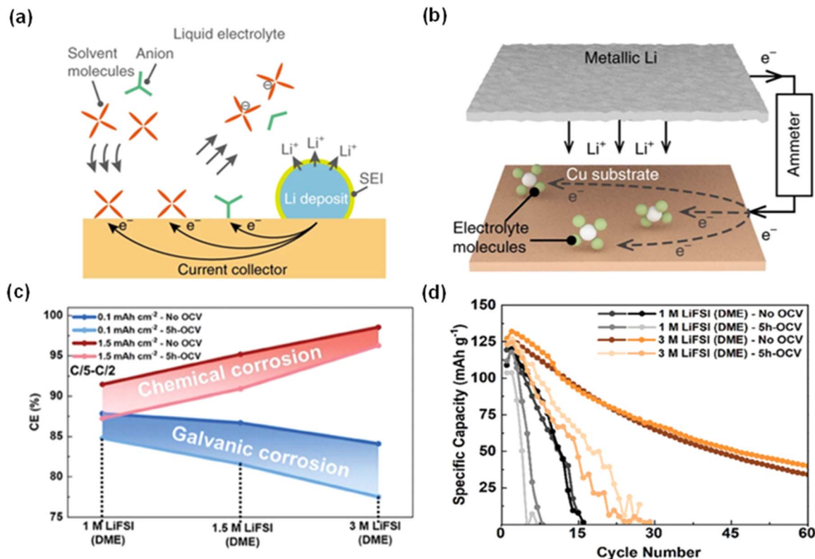
Fig. 2 Lithium galvanic corrosion and testing method. (a) The mechanism of galvanic corrosion through transporting electrons using a current collector. (b) The schematic of testing the galvanic corrosion. The current flow through an ammeter quantifies the corrosion rate of Li connected to the current collector. 16 Reproduced with permission. Copyright 2019, Springer Nature. (c) Average CEs of cells assembled with LiFSI (DME) of different concentrations and tested with a capacity of 0.1 or 1.5 \text{mA h cm}^{-2} . (d) Cycling performance of Cu||LCO employing 1 M LiFSI (DME) and 3 M LiFSI (DME) with and without a 5-hour open circuit voltage (OCV). 17 Reproduced with permission. Copyright 2023, Wiley-VCH.
