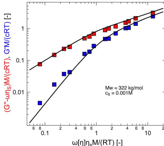
Fig. 6 Storage and loss modulus for sodium polystyrene sulfonate in 0.001 M NaCl salt solutions. Measurements at T = 5, 15, and 25\text{ }^{\circ}\text{C} were plotted into a single master-curve. Lines are the Zimm model using eqn (8.67) and (8.68) from ref. 86 with \nu = 0.59 . Data are from ref. 274.
