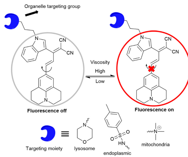
Fig. 14 Schematic view of viscosity response to an organelle targeting molecular rotor.
