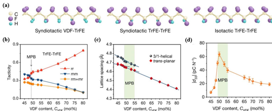
Fig. 9 (a) Schematic diagram showing the chain tacticity in P(VDF-TrFE). (b) Tacticity of the TrFE-TrFE segment as a function of VDF content. Data were given for the isotactic ( mm ), syndiotactic ( rr ) and heterotactic ( mr + rm ) configurations. (c) Intermolecular lattice spacing versus VDF content. The light-green-shaded area indicated the transition region, across which the structure changed abruptly. (d) Magnitude of d_{33} as a function of VDF content. This figure has been reproduced from ref. 114 with permission from Springer Nature, copyright 2018.
