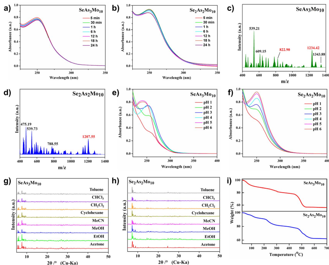
Fig. 2 (a) and (b) UV-vis spectra of aqueous solutions containing SeAs 3 Mo 10 and Se 2 As 2 Mo 10 at various time intervals. (c) and (d) Negative-ion mass spectra of SeAs 3 Mo 10 and Se 2 As 2 Mo 10 . (e) and (f) UV-vis spectra of the aqueous solution containing SeAs 3 Mo 10 and Se 2 As 2 Mo 10 at different pH conditions. (g) and (h) Powder XRD patterns of SeAs 3 Mo 10 and Se 2 As 2 Mo 10 after soaking in different organic solvents for 24 h. (i) Thermogravimetric curves of SeAs 3 Mo 10 and Se 2 As 2 Mo 10 .
