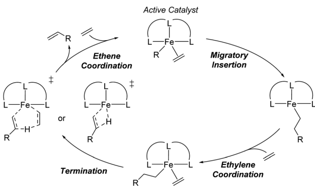
Scheme 1 General catalytic cycle for tridentate Fe-catalyzed ethene oligomerization.
