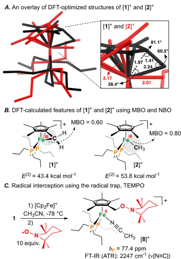
Fig. 6 (A) Structural overlay (capped sticks) of [1]^+ (black) and [2]^+ (red). Select angles ( ^\circ ) and select bond lengths ( \text{Å} ) are provided. (B) Mayer bond order (MBO) and natural bond orbital (NBO) analysis providing E^{(2)} values between \text{Fe}\text{--}\text{C} . (C) Reaction of [1]^+ with (2,2,6,6-tetramethylpiperidin-1-yl)oxyl (TEMPO) forming [8]^+ .
