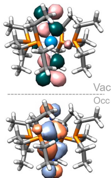
Fig. 11 NTOs (occupied – bottom, vacant – top) of the 450 nm band of the bare tungsten complex.
