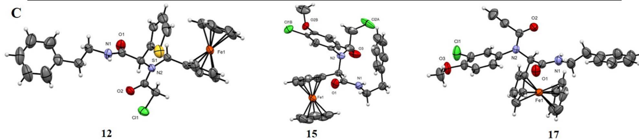
Fig. 2 (A) Illustration of the ferrocene-based organometallic compound library construction and screening. (B) Structure-based drug design (SBDD) of ferrocene-appended GPX4 inhibitors. (C) Molecular structures of the ferrocene complexes 12 , 15 and 17 with thermal ellipsoids shown at 50% probability.
