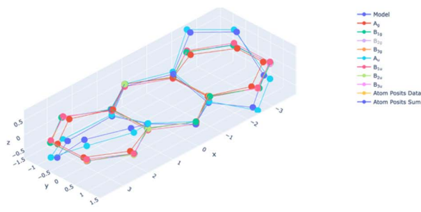
Figure 2: Atom positions and symmetric decomposition modes
