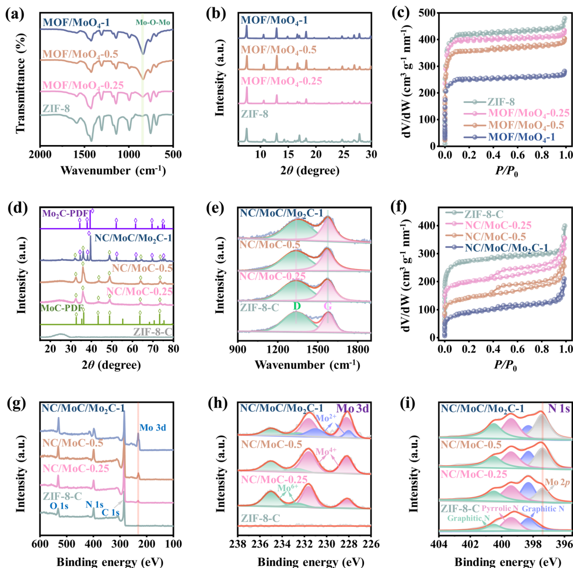
Fig. 2 (a) FTIR spectra, (b) XRD patterns, and (c) N_2 adsorption/desorption isotherms of the ZIF-8 RDs and MOF/ MoO_4 - x ( x = 0.25, 0.5 and 1 ). (d) PXRD patterns of MoC PDF#06-0546, Mo_2C PDF#35-0787, ZIF-8-C, NC/ MoC -0.25, NC/ MoC -0.5, and NC/ MoC / Mo_2C -1. (e) Raman spectra, (f) N_2 adsorption-desorption isotherms, (g) XPS survey spectra, and high-resolution XPS spectra of (h) Mo 3d and (i) N 1s of ZIF-8-C, NC/ MoC -0.25, NC/ MoC -0.5, and NC/ MoC / Mo_2C -1.
