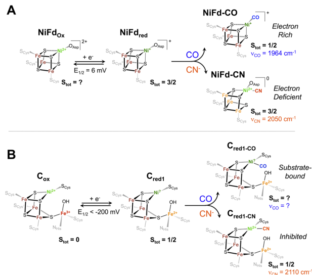
Fig. 8 Proposed electronic and geometric structures of the (A) \text{NiFd}_{\text{ox}} , \text{NiFd}_{\text{red}} , \text{NiFd-CO} , and \text{NiFd-CN} species with key experimental metrics indicated that have been obtained from this work, and (B) analogous \text{C}_{\text{ox}} , \text{C}_{\text{red1}} , \text{C}_{\text{red1-CO}} , and \text{C}_{\text{red1-CN}} states of CODH with spectroscopic metrics obtained from ref. 17, 75 and 76.
