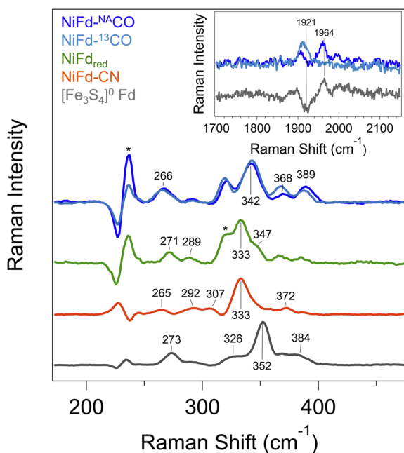
Fig. 4 Resonance Raman spectra of [\text{Fe}_3\text{S}_4]^0 Fd (gray), NiFd red (green), NiFd-CN (orange), and NiFd-CO (blue). Samples were collected at 77 K using an excitation wavelength of 407 nm, P = 8\text{ mW} . Residual features corresponding to buffer are indicated with an *. Bands arising from buffer, DT, and quartz were subtracted after collection. (Inset) High frequency region of the resonance Raman spectra of NiFd-CO prepared with natural abundance CO (dark blue) and ^{13}\text{C} O (light blue), shown offset from the difference spectrum (gray). The band at 1906\text{ cm}^{-1} is present in both samples and independent of the CO isotope.
