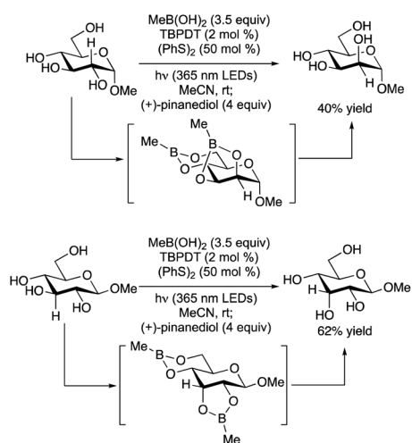
Scheme 61 Methylboronic acid-mediated photocatalytic trans -to- cis diol epimerization of glucopyranosides. DBPDT denotes tetrabutylphosphonium decatungstate, [\text{Bu}_4\text{P}^+]_4[\text{W}_{10}\text{O}_{32}]^{4-} .
