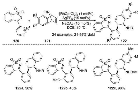
Scheme 35 Synthesis of ADHNs via rhodium(III)-catalyzed ring-opening addition reaction of azabenzonornorbornadienes with N -sulfonyl ketimines.
