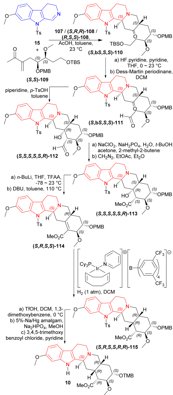
Scheme 30 Total synthesis of (+)-reserpine by primary amine catalysts and [Ir(COD)(PCy 3 )(py)]BAR F .
