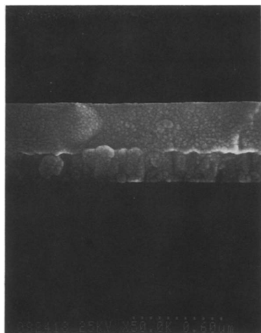
Fig. 4 Cross-section of \text{Ta}_2\text{O}_5 thin film prepared by the sol-gel method using photo-irradiation (Reproduced from ref. 44 with permission from Elsevier copyright [2024]).
