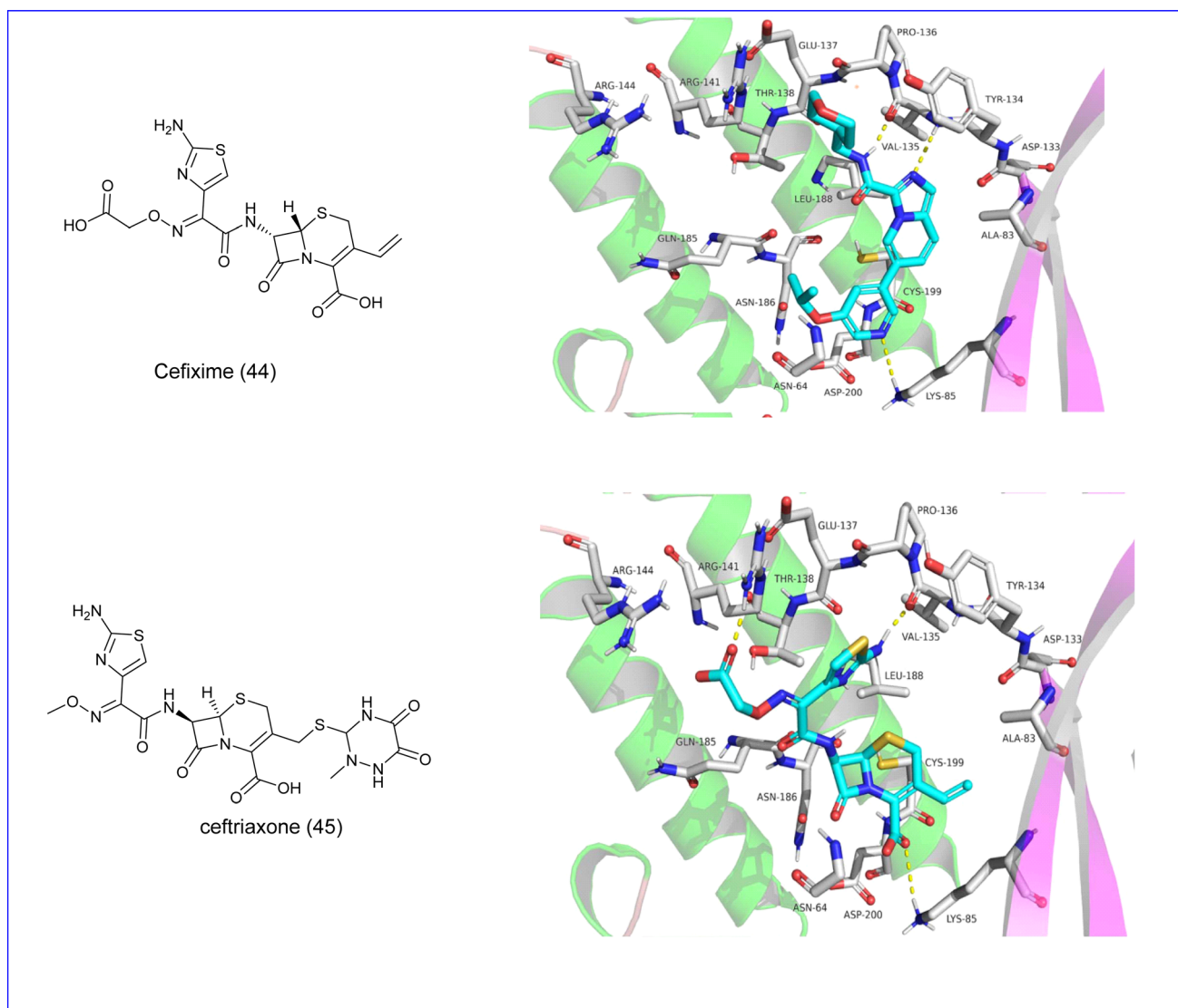
Fig. 29 (A) Molecular docking of cefixime ( 44 ) GSK3 protein. (B) Molecular docking of ceftriaxone ( 45 ) with GSK3 protein.
