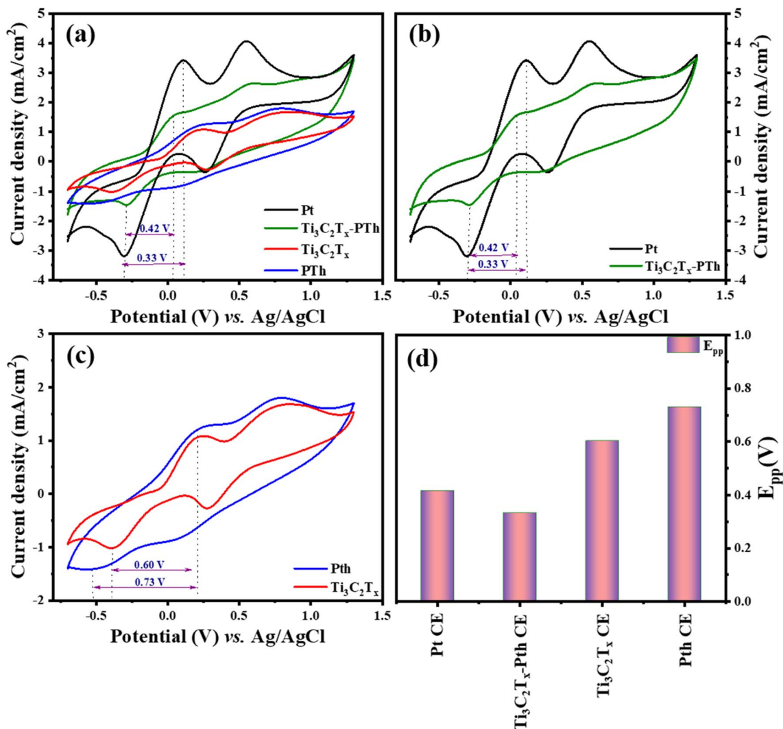
Fig. 5 Cyclic voltammograms of (a) Pt, Ti_3C_2T_x , Pth, Ti_3C_2T_x -Pth at 50 mV s^{-1} scan rate (b–d) comparison of cyclic voltammograms Pt and Ti_3C_2T_x -Pth CEs, Ti_3C_2T_x and Pth CEs, and overall E_{pp} comparison of Pt, Ti_3C_2T_x , Pth, Ti_3C_2T_x -Pth CEs.
