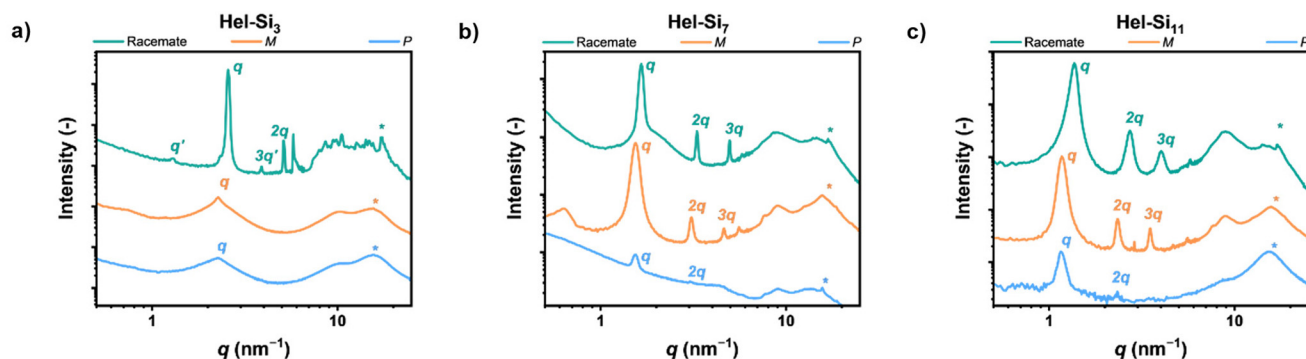
Fig. 3 MAXS/WAXS spectra of the rac -, P - and M -forms of Hel-Si 3 (a), Hel-Si 7 (b) and Hel-Si 11 (c). It should be noted that the curves of P - Hel-Si n are recorded on Kapton tape due to the small amount synthesized and therefore differences with the enantiomer M - Hel-Si n are observed due to the different processing conditions and the lower sensitivity of the measurement.
