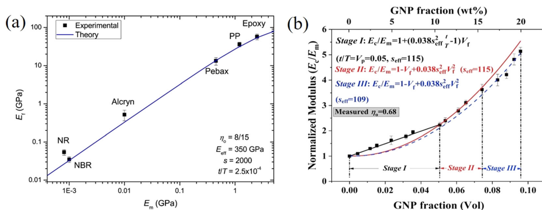
Fig. 19 (a) Variation of the modulus of graphene nanoplatelets (GNPs) with the modulus of the matrices (dots: experimental data; blue line: theory predictions from eqn (16) and (19)). Reproduced with permission from ref. 171. Copyright 2018 Elsevier. (b) Three stages for the reinforcement of GNPs on elastomers. Reproduced with permission from ref. 153. Copyright 2019 Elsevier.
