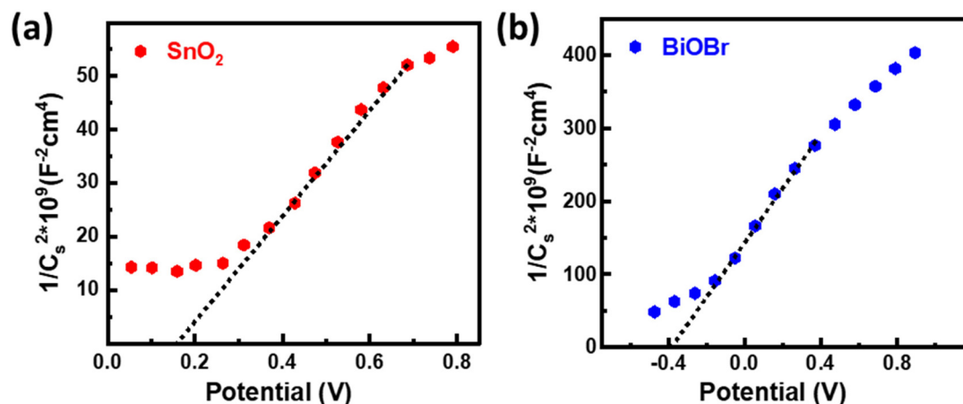
Fig. 9 Mott-Schottky plots for (a) SnO 2 and (b) BiOBr.
