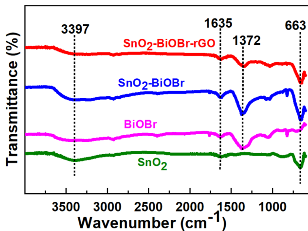
Fig. 2 FTIR spectra for \text{BiOBr} , \text{SnO}_2 , \text{SnO}_2\text{-BiOBr} , and \text{SnO}_2\text{-BiOBr-rGO} .
