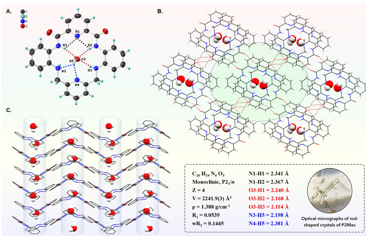
Fig. 2 SC-XRD analysis of \text{P2Mac} \cdot \text{H}_2\text{O} . (A) ORTEP diagram at 50% probability showing intermolecular H-bonding interactions of P2Mac with \text{H}_2\text{O} . (B) Crystal packing along the b -axis: a top-view perspective highlighting intermolecular short-contact interactions. (C) Crystal packing along the a -axis illustrating the formation of linear stacks of water molecules in the crystals to form water channels for proton conduction (H atoms are omitted for clarity).
