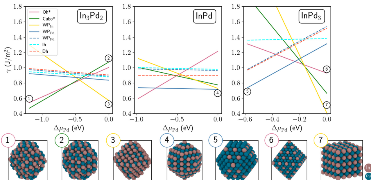
Fig. 5 Surface energies of In 3 Pd 2 (left), InPd (middle) and InPd 3 (right) NPs as a function of \Delta\mu_{\text{Pd}} = \mu_{\text{Pd}} - \mu_{\text{Pd}}^{\text{b}} . Chemically ordered and disordered NPs are shown with full and dashed lines, respectively. Colour code: Pd = blue and In = brown.
