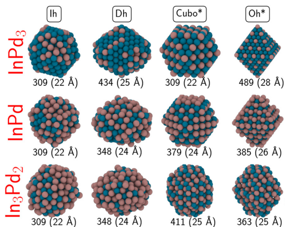
Fig. 4 Non-crystalline (Ih and Dh) and crystalline (Oh* and Cubo*) morphologies of In 3 Pd 2 , InPd and InPd 3 NPs. The diameter of each NP is given, along with its number of atoms. Colour code: Pd = blue and In = brown.
