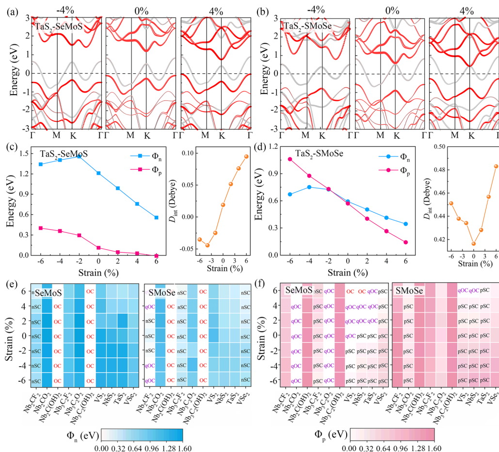
Fig. 7 The projected band structures of (a) \text{TaS}_2 -SeMoS and (b) \text{TaS}_2 -SMoSe contacts with different in-plane biaxial strains. Schottky barriers and interface dipole of (c) \text{TaS}_2 -SeMoS and (d) \text{TaS}_2 -SMoSe as a function of biaxial strains. Schottky barrier heights (e) \Phi_n and (f) \Phi_p of 2D metal-SeMoS and metal-SMoSe contacts with different biaxial strains. OC means Ohmic contact, qOC means quasi-Ohmic contact ( \Phi_n or \Phi_p < 0.05 eV), nSC and pSC represent n-type and p-type Schottky contacts, respectively.
