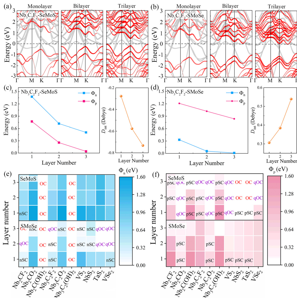
Fig. 6 The projected band structures of (a) Nb 3 C 2 F 2 -SeMoS and (b) Nb 3 C 2 F 2 -SMoSe contacts with monolayer, bilayer, and trilayer MoSe. Schottky barriers and interface dipole of (c) Nb 3 C 2 F 2 -SeMoS and (d) Nb 3 C 2 F 2 -SMoSe contacts as a function of MoSe layer number. Schottky barrier heights (e) \Phi_n and (f) \Phi_p of 2D metal-MoSe contacts with different MoSe layer numbers. OC means Ohmic contact, qOC means quasi-Ohmic contact ( \Phi_n or \Phi_p < 0.05 eV), nSC and pSC represent n-type and p-type Schottky contacts, respectively.
