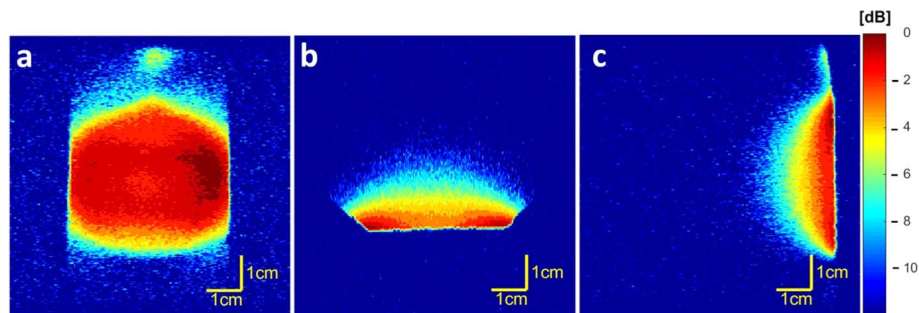
Fig. 1 Coil homogeneity measured using ^1\text{H} MRI at 4.7 T scanner in (a) coronal (b) axial and (c) sagittal planes; the color scale reflects signal attenuation (dB) – from the lowest (red) to the highest (blue).
