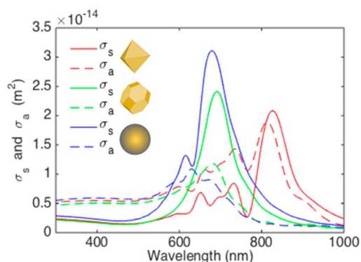
Fig. 21 Scattering (solid lines) and absorption (dashed lines) cross-sections vs. wavelength for different shaped nanoparticles of similar size embedded in a PCDTBT:PC 70 BM background. Red: 70 nm octahedral AuNPs. Green: 70 nm truncated octahedral AuNPs. Blue: 70 nm AuNSs. Reproduced from ref. 100 with permission from the American Chemical Society (CC BY-NC 4.0).
