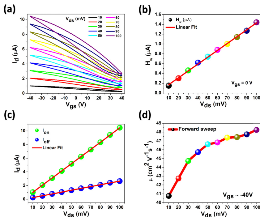
Fig. 3 (a) Transfer characteristics, (b) hysteresis width, (c) on and off current values at V_{\text{gs}} = -40 \text{V} and V_{\text{gs}} = 40 \text{V} , respectively, and (d) calculated mobility as a function of the drain voltage at V_{\text{gs}} = -40 \text{V} , RT and 2 mbar pressure. Line in (d) is guide to the eye.
