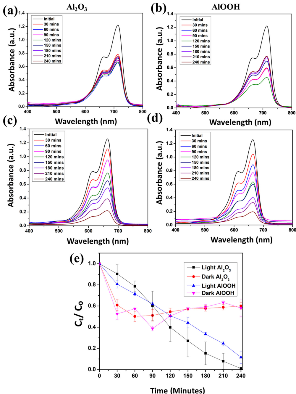
Fig. 6 UV-vis spectra of MB with Al 2 O 3 (a) and AIOOH (b) in the dark and Al 2 O 3 (c) and AIOOH (d) in the light at pH 9. Average degradation efficiency over time at pH 9 (e).
