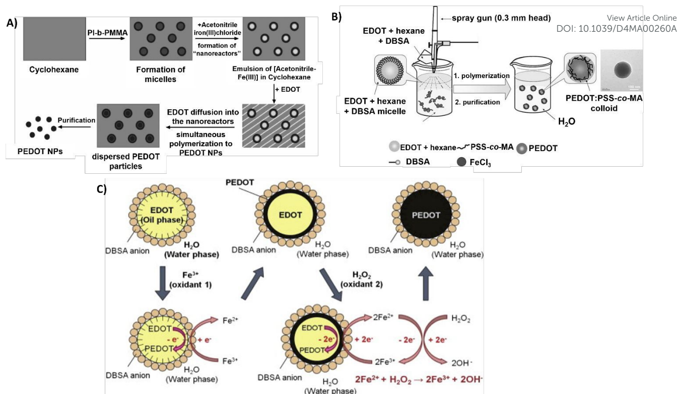
Fig. 3 Different polymerisation synthesis approaches of PEDOT NPs. A) PI- b -PMMA stabilised NPs in non-aqueous emulsion with cyclohexane and acetonitrile. Reproduced with permission from ref. 60 . Copyright 2006 Wiley. B) Spray emulsion polymerisation of PSS-co-MA stabilised PEDOT NPs. Reproduced with permission from ref. 63 . Copyright 2010 Wiley. C) Fe 3+ /H 2 O 2 bi-oxidant system. Reproduced with permission from ref. 67 . Copyright 2011 Elsevier.
