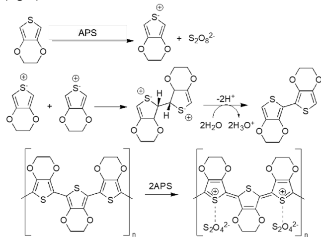
Fig. 2 Oxidative polymerisation of EDOT using APS as oxidising agent 68
