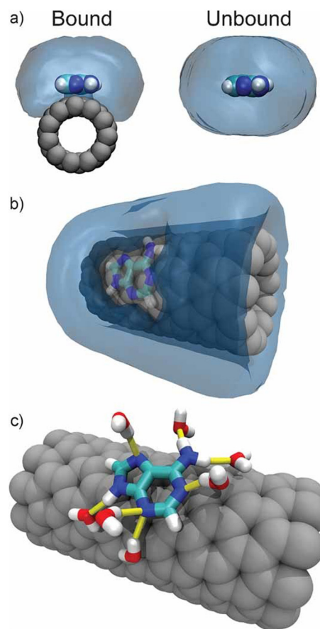
Fig. 4 (a) Water density around bound and unbound DNA (b) water density around CNT showing water excluded from the CNT surface due to the presence of the bound DNA (c) water remains capable of forming hydrogen bonds (yellow) with bound DNA. Reproduced from ref. 39 with permission from John Wiley and Sons, copyright 2009.
