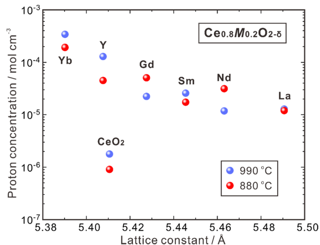
Fig. 3 Proton concentration in undoped \text{CeO}_2 and \text{Ce}_{0.8}\text{M}_{0.2}\text{O}_{2-\delta} ( M = \text{Y, La, Nd, Sm, Gd, Yb} ) after annealing at 880 and 990 °C in a wet atmosphere ( p_{\text{H}_2\text{O}} = 0.03 \text{ atm} ). 62
