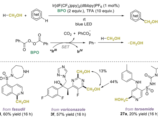
Fig. 32 Photoredox Minisci hydroxymethylation with methanol.
