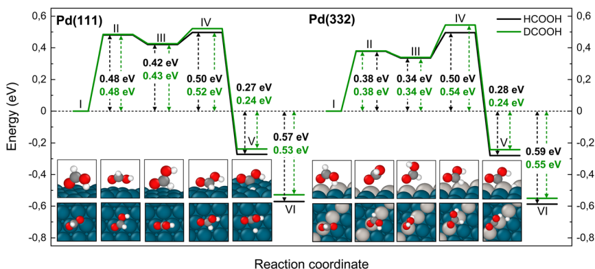
Fig. 5 Reaction pathway for carboxyl formation from HCOOH (black) and from DCOOH (green) on Pd(111) and Pd(332) obtained from NEB calculations using PBE-TS functional. On the scheme the initial state (I), the first transition state (II), the intermediate state (III), the second transition state (IV) and the final state (V) are shown. Energy level VI corresponds to final state V without interaction between products. Atom representation is the same as in Fig. 4. The energy values include ZPE correction.
