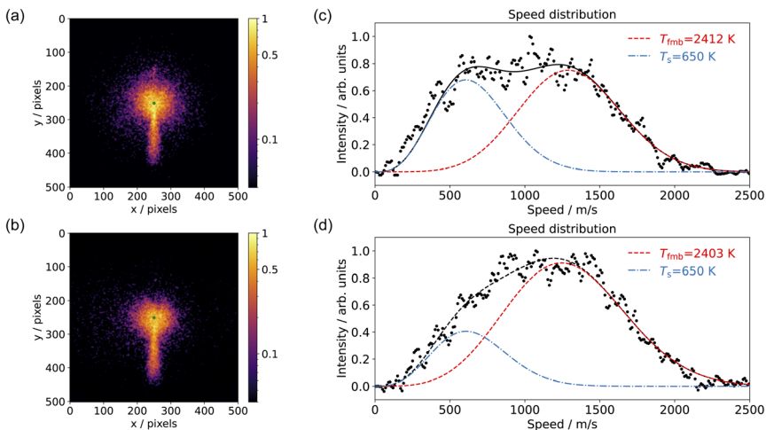
Fig. 4 Comparison of the velocity-map images of CO 2 from CO oxidation on Pd(110) at T_s = 650\text{ K} and (a) a pure CO beam with p_{\text{O}_2} = 7.5 \times 10^{-8}\text{ mbar} ; (b) a 10% O 2 in He beam with p_{\text{CO}} = 5 \times 10^{-6}\text{ mbar} in the scattering chamber. The green dot in (a) and (b) represents the center of the image (zero velocity). (c) and (d) show the corresponding speed distributions (black dots) for CO 2 from (a) and (b), respectively. The speed distribution is fitted (black dashed) with one slow component (blue dashes) and one fast component (red dashes).
