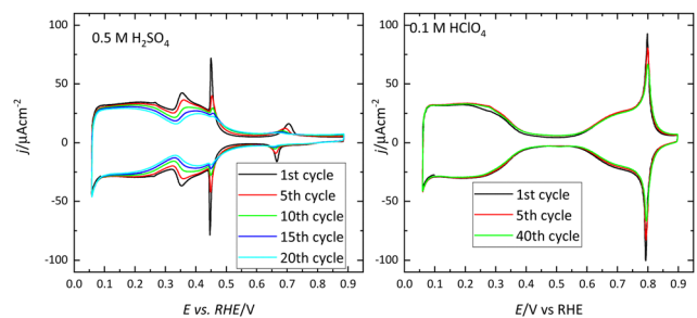
Fig. 2 Evolution upon cycling of the voltammetric profiles of a Pt(111) electrode in 0.5 M \text{H}_2\text{SO}_4 and 0.1 M \text{HClO}_4 with different levels of impurities. Scan rate: 50 \text{ mV s}^{-1} .
