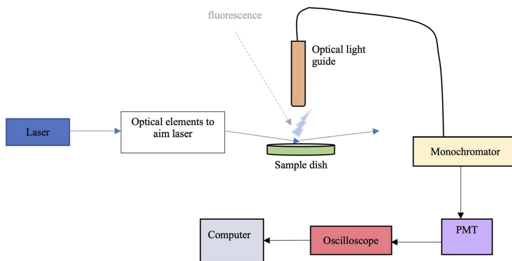
Fig. 2 Box diagram of the glancing-angle laser-induced fluorescence instrument setup.
