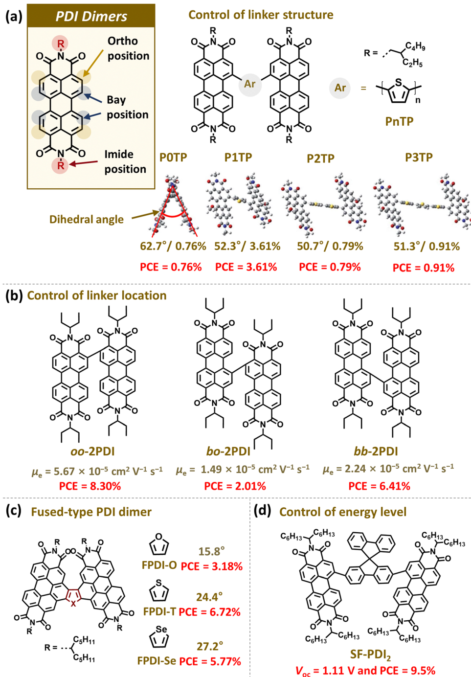
Fig. 5 Representative examples of PDI-based dimer acceptors; (a) P0TP, P1TP, P2TP, and P3TP, (b) oo-2PDI, bo-2PDI, and bb-2PDI, (c) FPDl-O, FPDl-T, and FPDl-Se, and (d) SF-PDI 2 . Reproduced from ref. 121 with permission from the Royal Society of Chemistry, copyright 2024.
