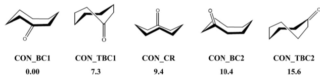
Scheme 2 Five low-energy CON conformers as reported in ref. 28. We have also given their relative energies (in \text{kJ mol}^{-1} ) with respect to the most stable one.
