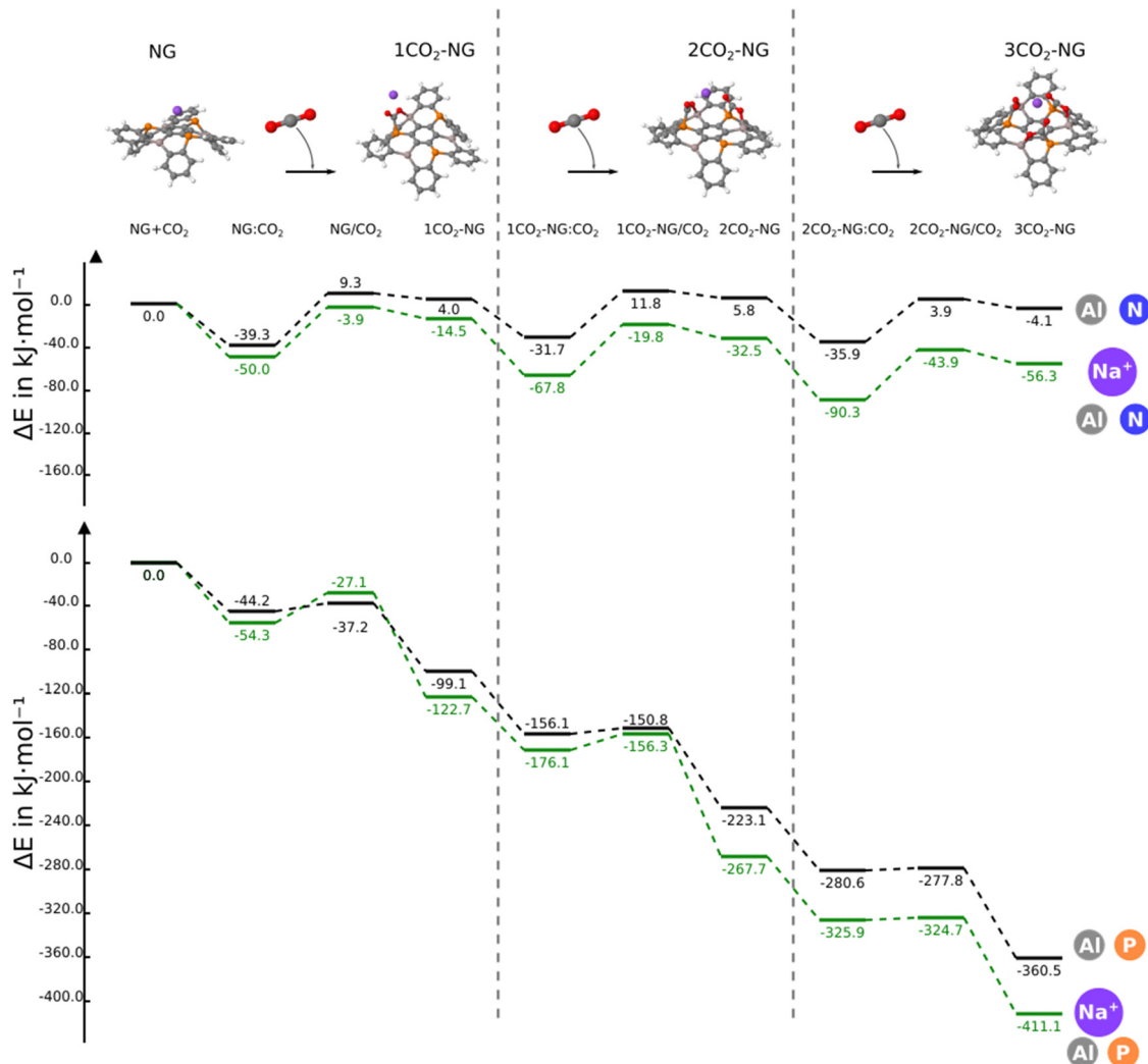
Fig. 8 Comparative energy profiles for the reaction of Al 3 N 3 -NG and Al 3 P 3 -NG in the absence/presence of Na + with three CO 2 molecules.
